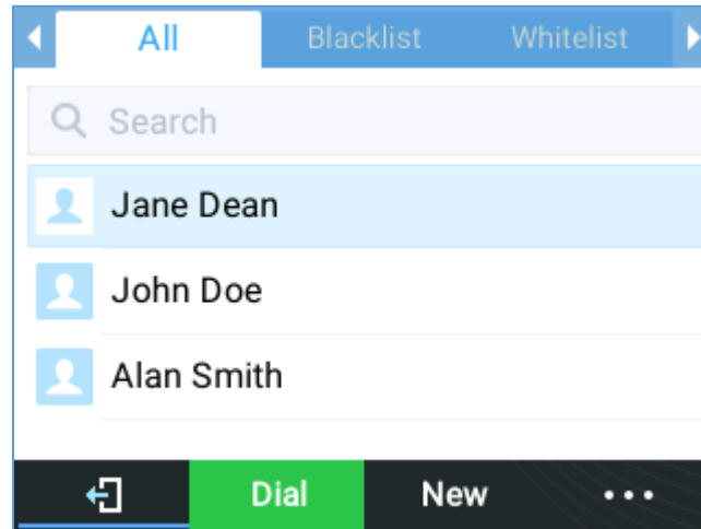
Figure 67: Before Search
