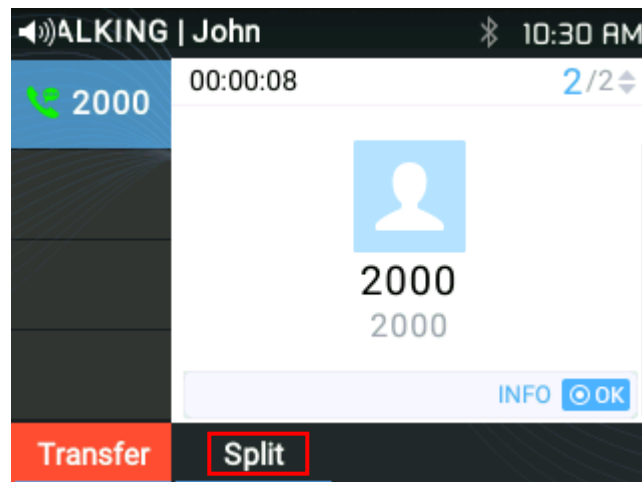
Figure 26: "Split" softkey
