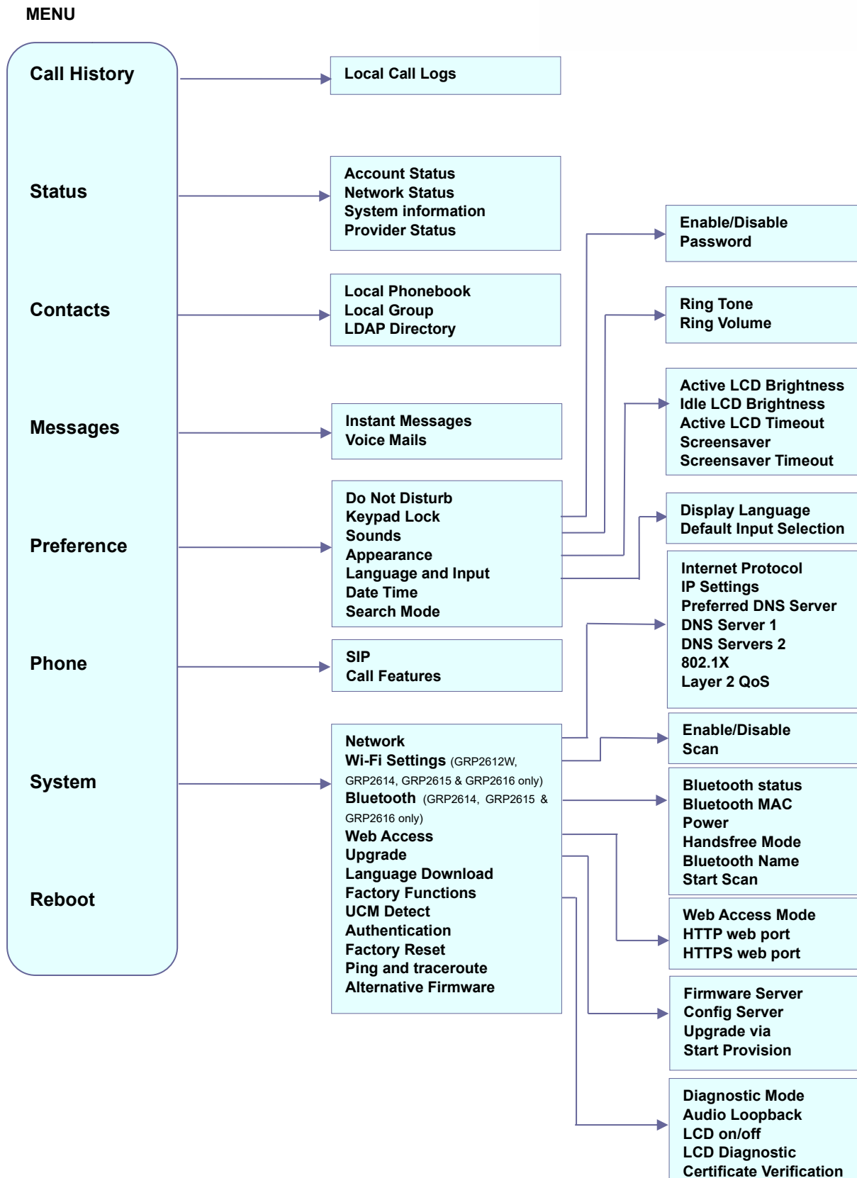
Figure 11: GRP261X Menu
