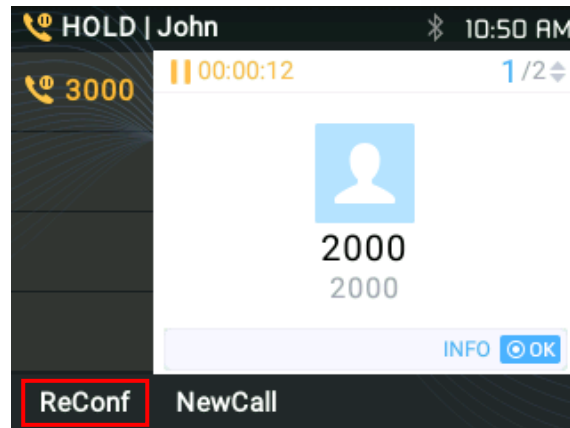
Figure 32 : Split conference
