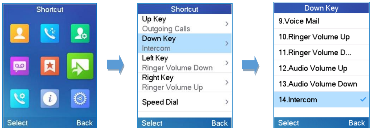
Figure 39: Shortcut Setting
